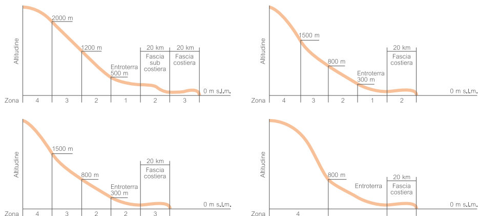
Fig. 5: Suddivisione del territorio nazionale in zone climatiche (circa. Min. LL.PP. n; 22631 del 24. 05. 82. Fig. 5: Division of the Italian national territory into climate zones (Min. Public Works, circular no. 22631 of 24.05. 82.
